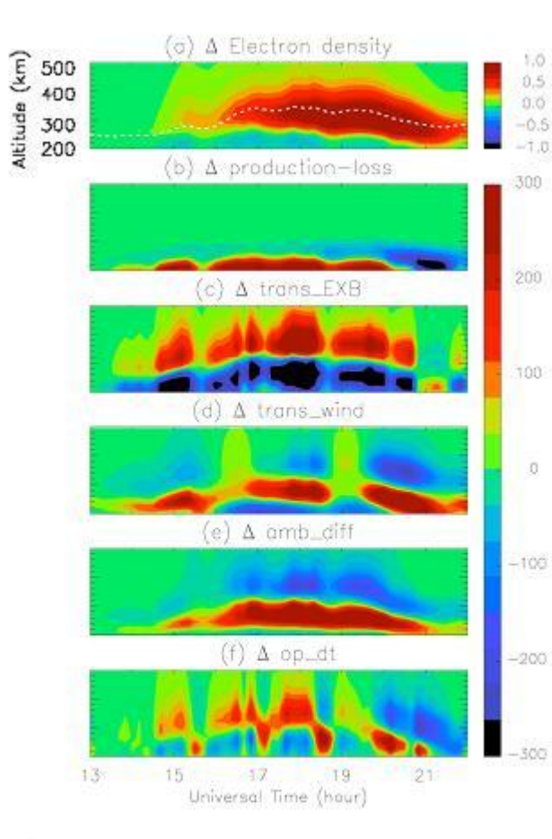
Figure (1) a time series showing events before and during a space weather event impacting the ionosphere.
